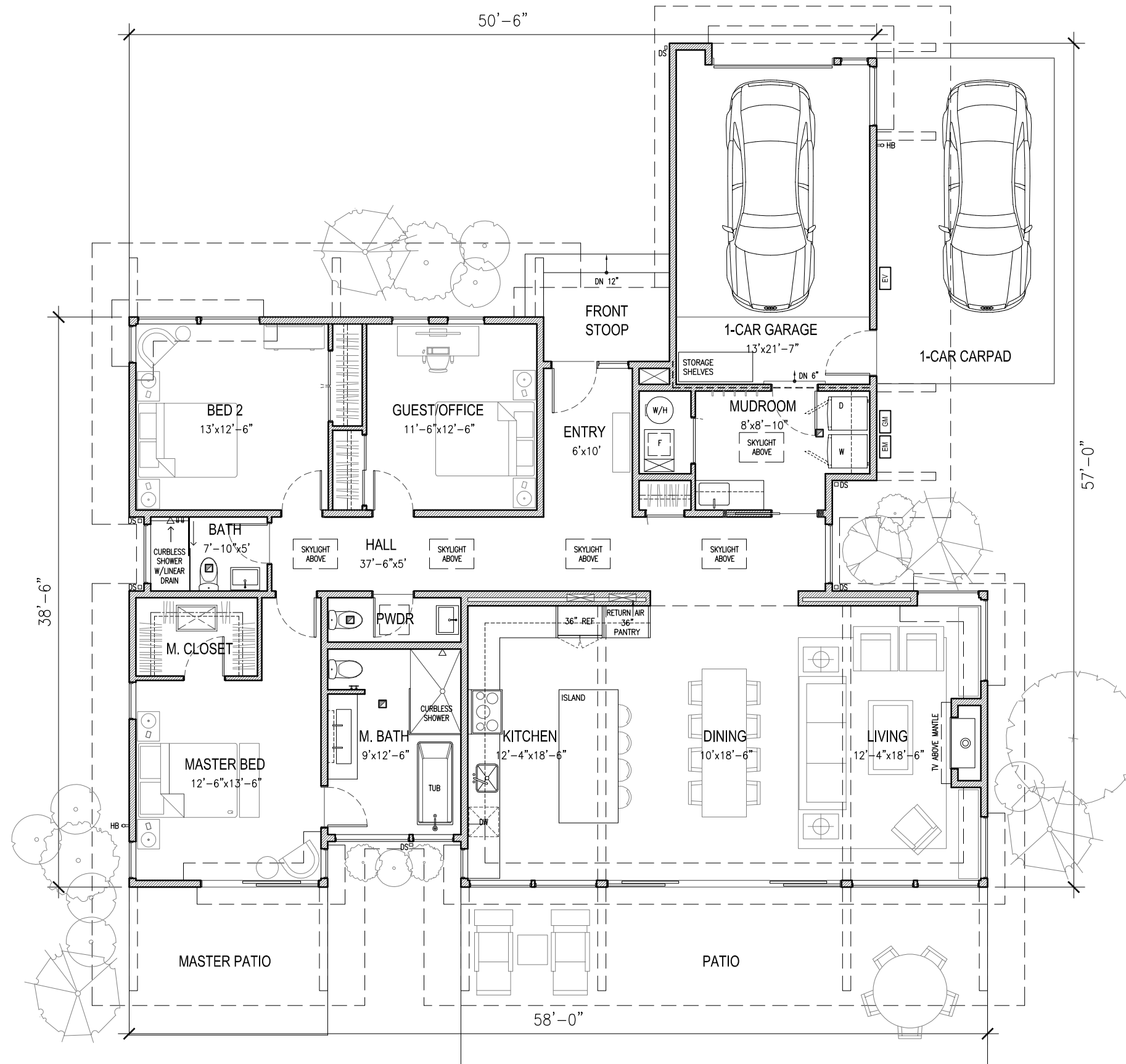
sd143 Modified Floor Plan - 1943 sf (heated)
