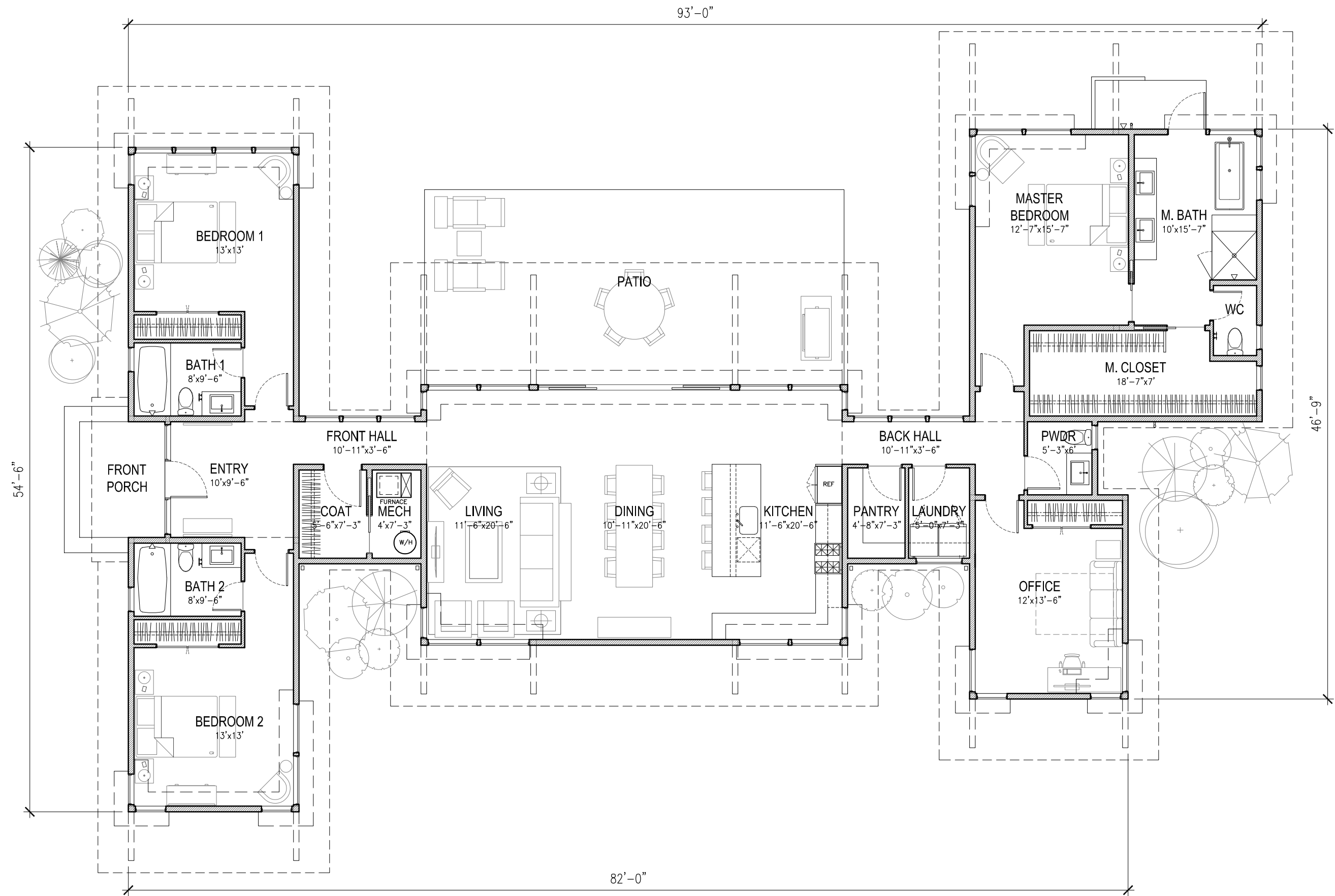
sd171 Modified Floor Plan - 2,582 sf
